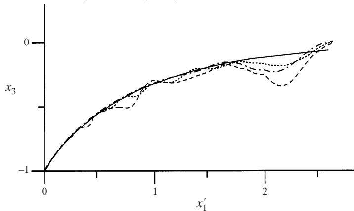
FIGURE 13. (Instantaneous) front shape of gravity currents advancing over slip boundaries (same flow fields as in figure 12). Results for -\cdot-\cdot- , Gr = 2 \times 10^7 ; --- , 4 \times 10^8 ; — , 2 \times 10^9 . The solid line shows the front given by Benjamin (1968).
